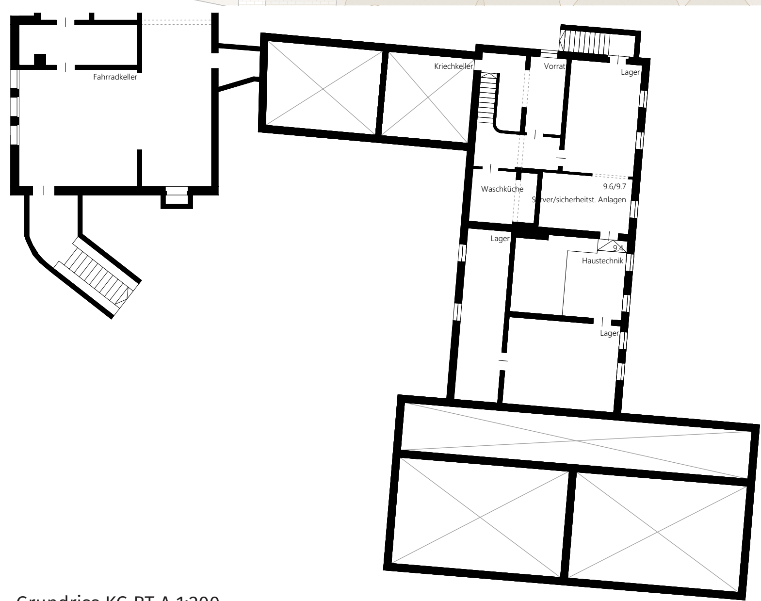
Grundriss KG BT A 1:200
